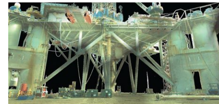
SafScan™ of Noble Max Smith oil rig.
