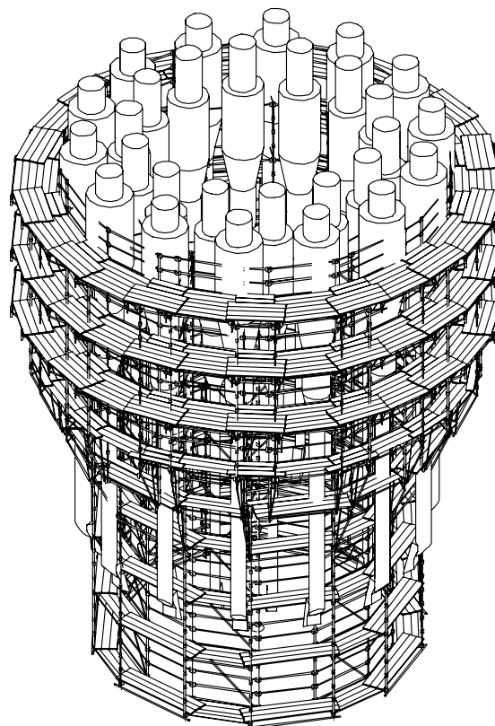
A jig stand engineered with Systems™ Scaffold
